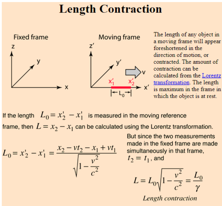
Fig.2. Consequences from Lorentz transformations: length contraction in a moving system/frame.
