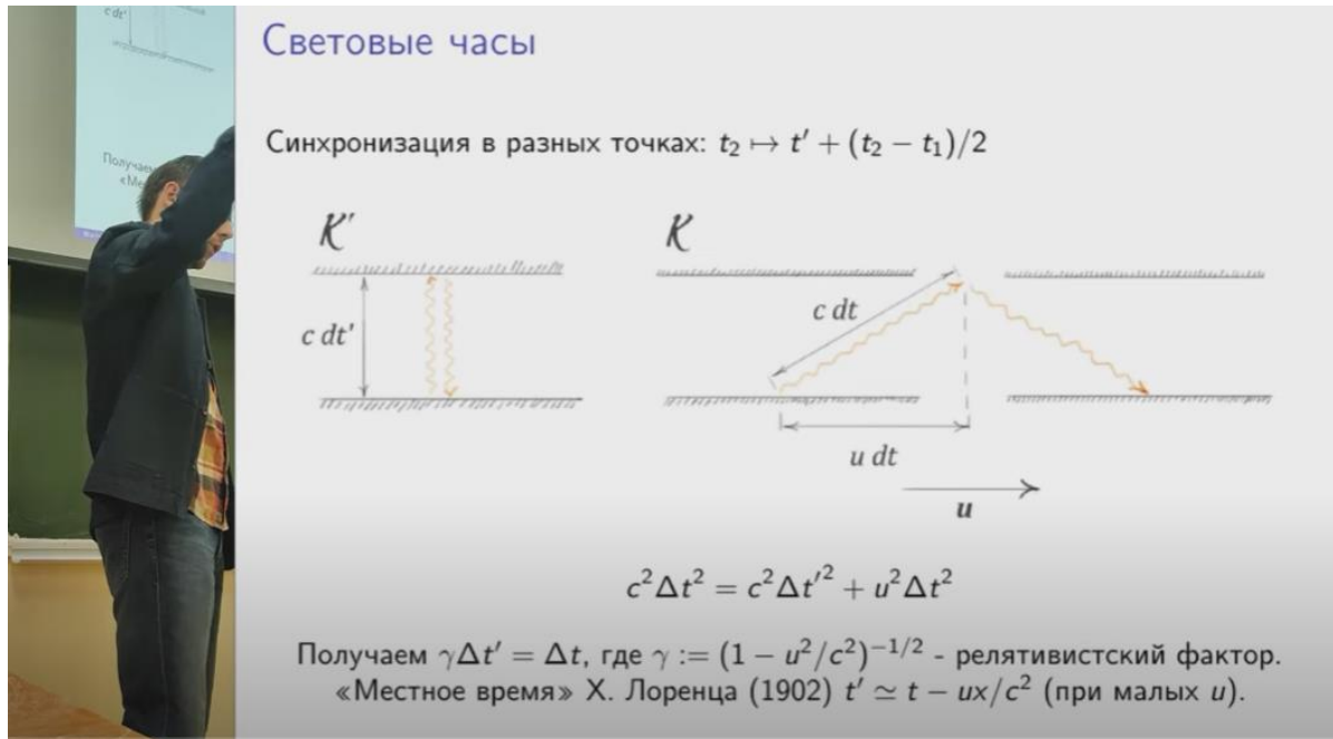
Fig. 3. Trajectories of light in light clocks in a stationary frame K' and a moving frame K . And deduction of Lorentz factor which is used extensively later in many “relativist equations”.
