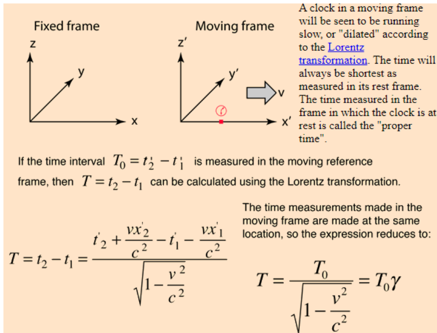
Fig. 1. Consequences from Lorentz transformations: time dilation in a moving system/frame.
